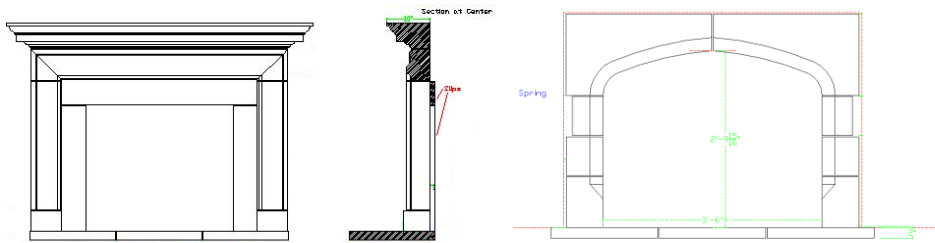
Config G (Camden) with Overmantle Note: shown with slips
