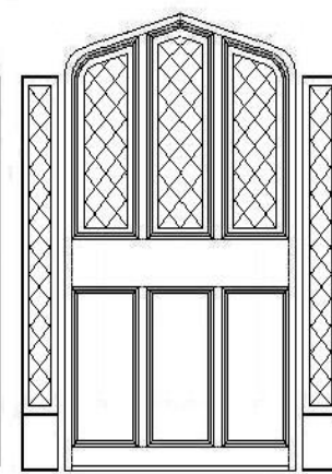
Tudor Panel, half-lighted, sidelight
