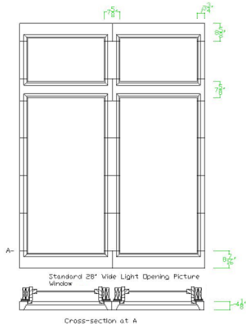
Half Mullion 4-light System
