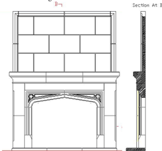
Config C with Overmantle
