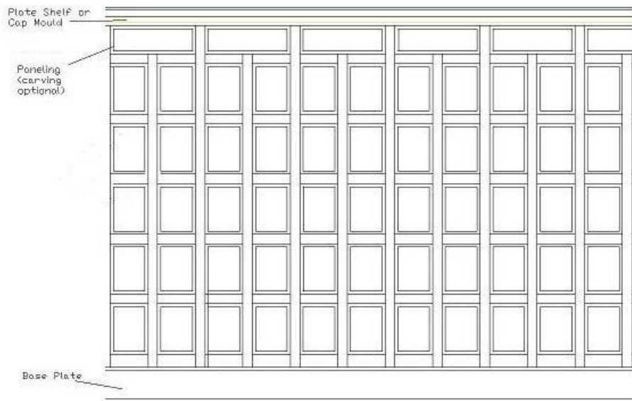
TYPICAL TUDOR PANELING
