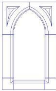
Gothic Window with Gordon Profile, Recessed Spandrels
